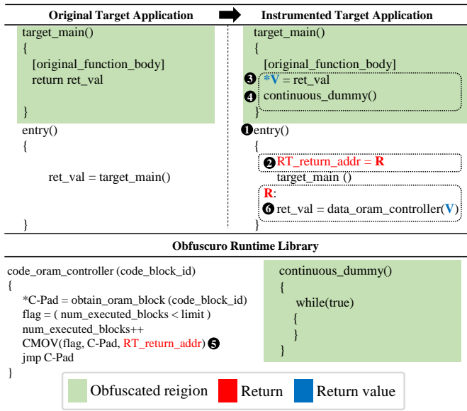
Fig. 7: OBFUSCURO’s continuous execution.
