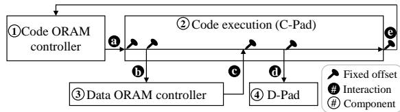
Fig. 8: Data oblivious execution cycle of OBFUSCURO
